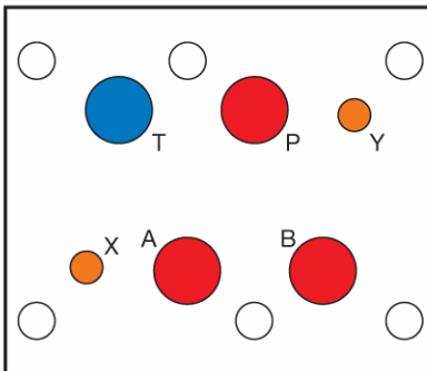
CETOP 7, 8 e 10 – TN16, 26 3 32
